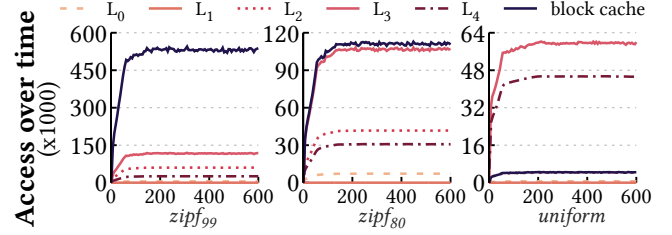
Figure 5: Read operations done over time (in seconds) across LSM levels under different data distributions.
