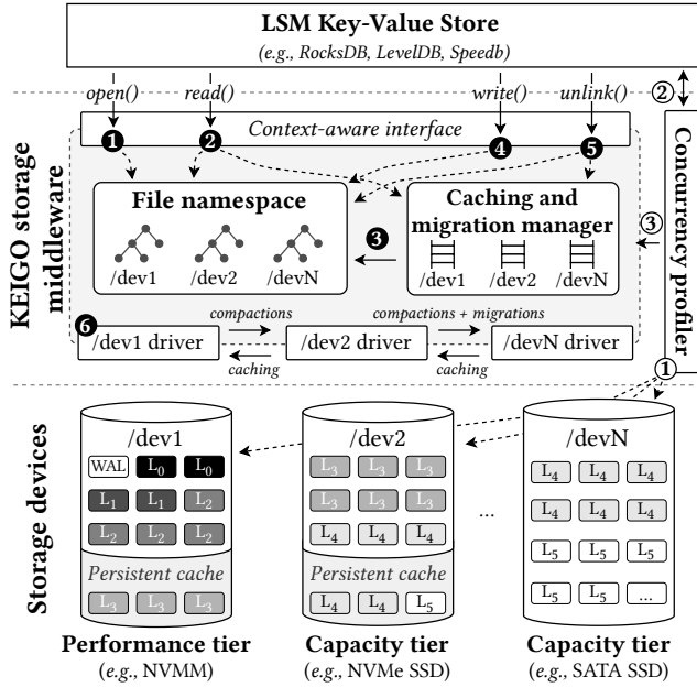
Figure 6: KEIGO architecture. It follows a multi-tier storage hierarchy, co-designed with the properties of LSM KVS and the inherent characteristics of different storage devices.
