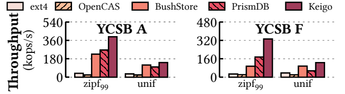
Figure 9: Performance under strict durability.
