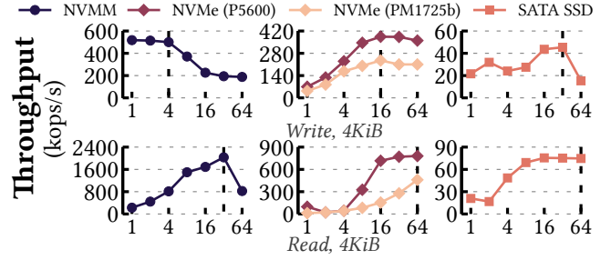
Figure 1: Performance of NVMM, two NVMe SSDs, and SATA SSD storage devices for FIO write and read workloads with increasing number of threads (1 to 64, x-axis). Vertical lines mark the maximum performance achieved by each device.
