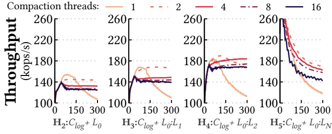
Figure 4: RocksDB performance over time (in seconds) under different placement schemes with increasing number of concurrent compactions. The caption of each plot depicts the components placed on NVMM.
