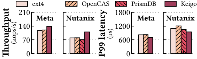
Figure 11: Performance of ext4 , OpenCAS , PrismDB , and KEIGO under Meta and Nutanix production workloads.
