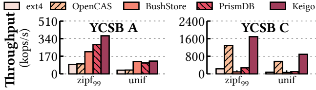
Figure 8: Performance under direct I/O for YCSB A and C.
