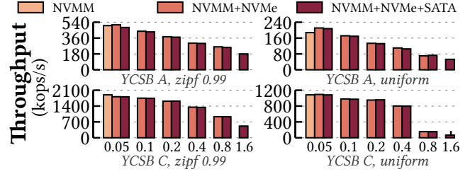
Figure 14: Performance with different tiers and dataset sizes.
