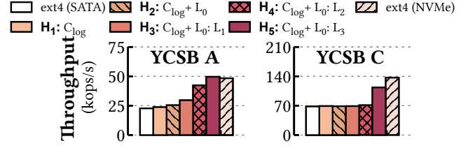
Figure 3: RocksDB performance when placing LSM components across an NVMe-SATA SSDs hierarchy under mixed and read-only workloads.
