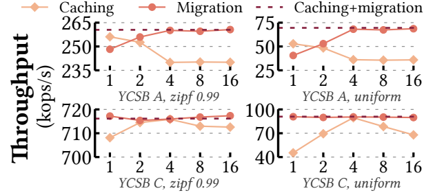
Figure 15: Performance of KEIGO’s automatic thread control for caching and migrations.
